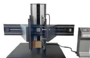
GT-N55 Packing Clamping Force Tester
